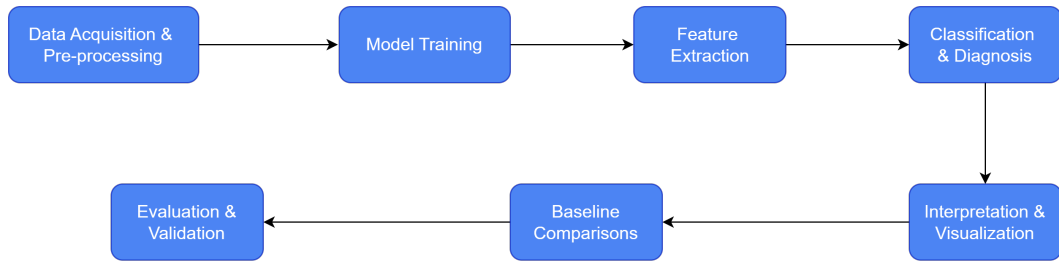
Figure 3.1: Overall Methodology
